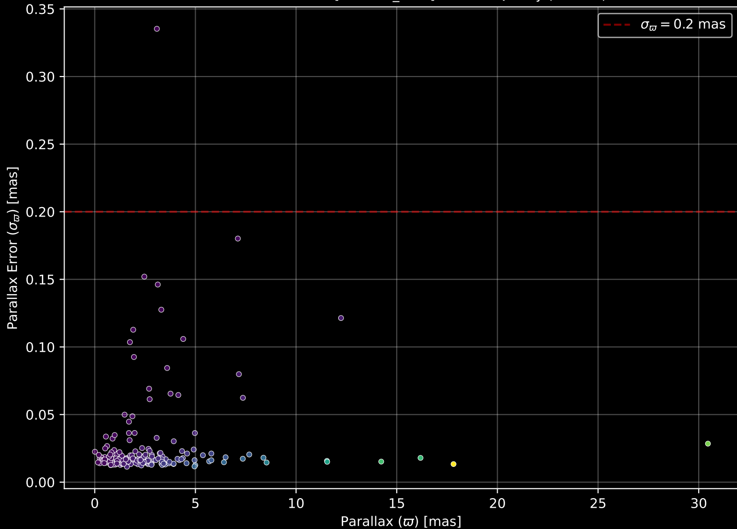
APOGEE DR17 Field: [175+31_MGA] Parallax Quality (n= 187)
