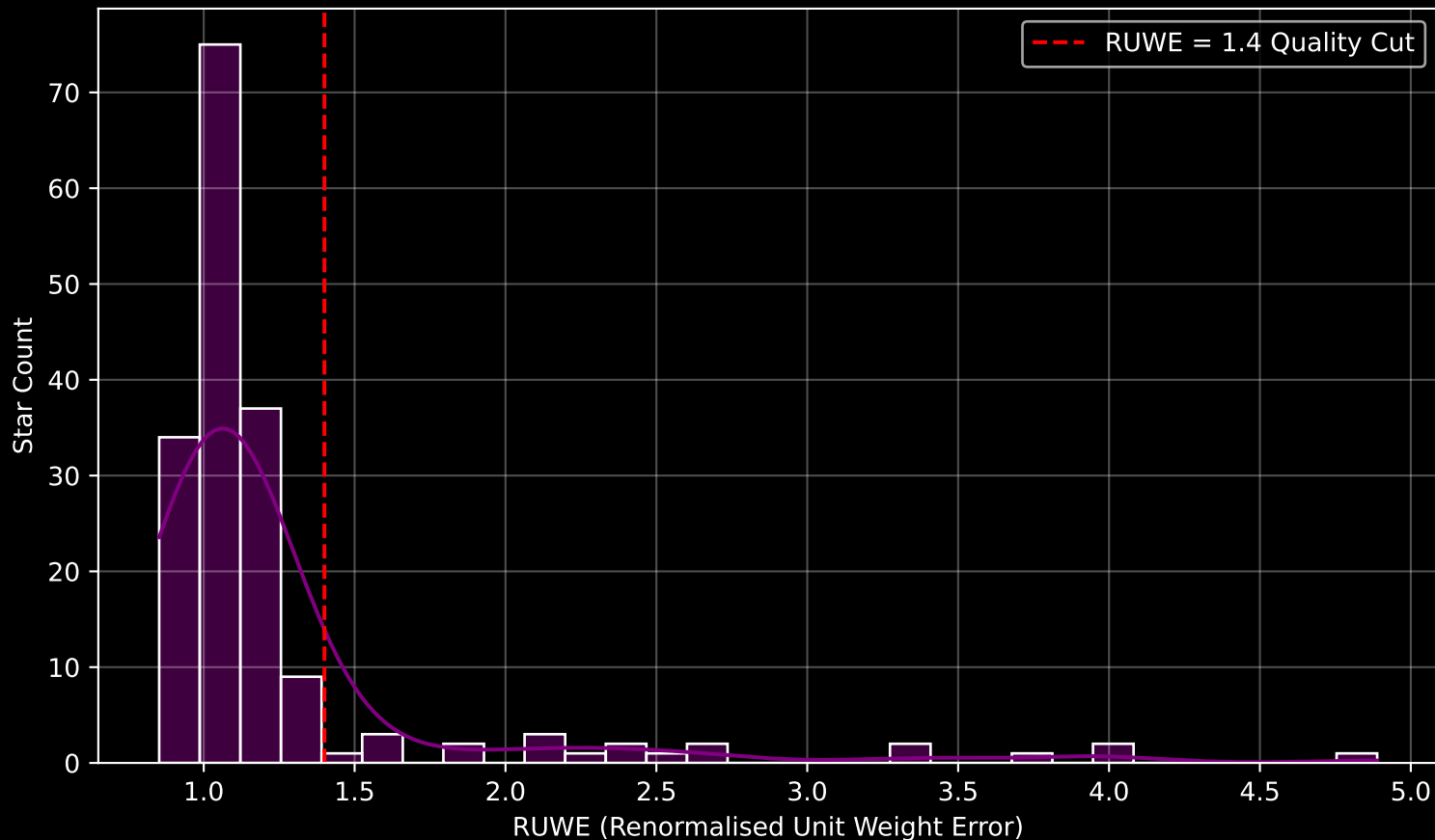
GAPOGEE DR17 Field [175+31_MGA] RUWE Distribution (n= 176)
