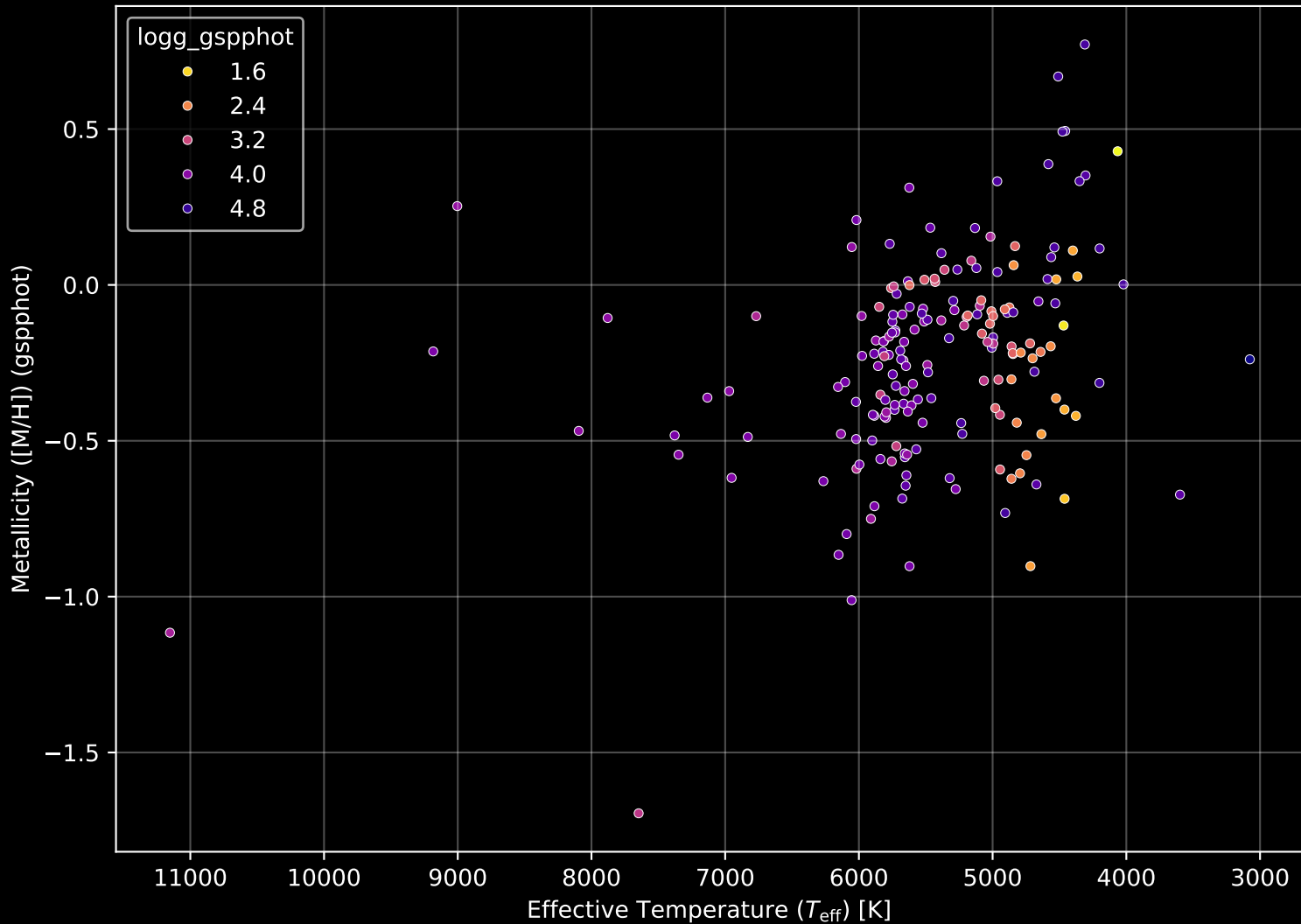
APOGEE DR17 Field: [175+31_MGA] Stellar Population Parameters (n= 187)
