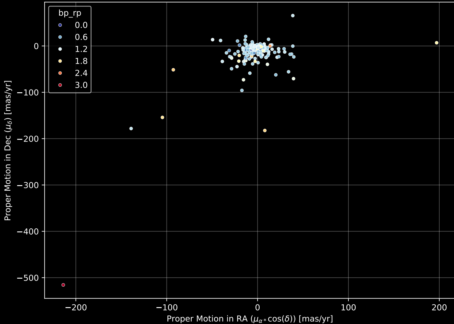
APOGEE DR17 Field: [175+31_MGA] Proper Motion Diagram (n= 187)
