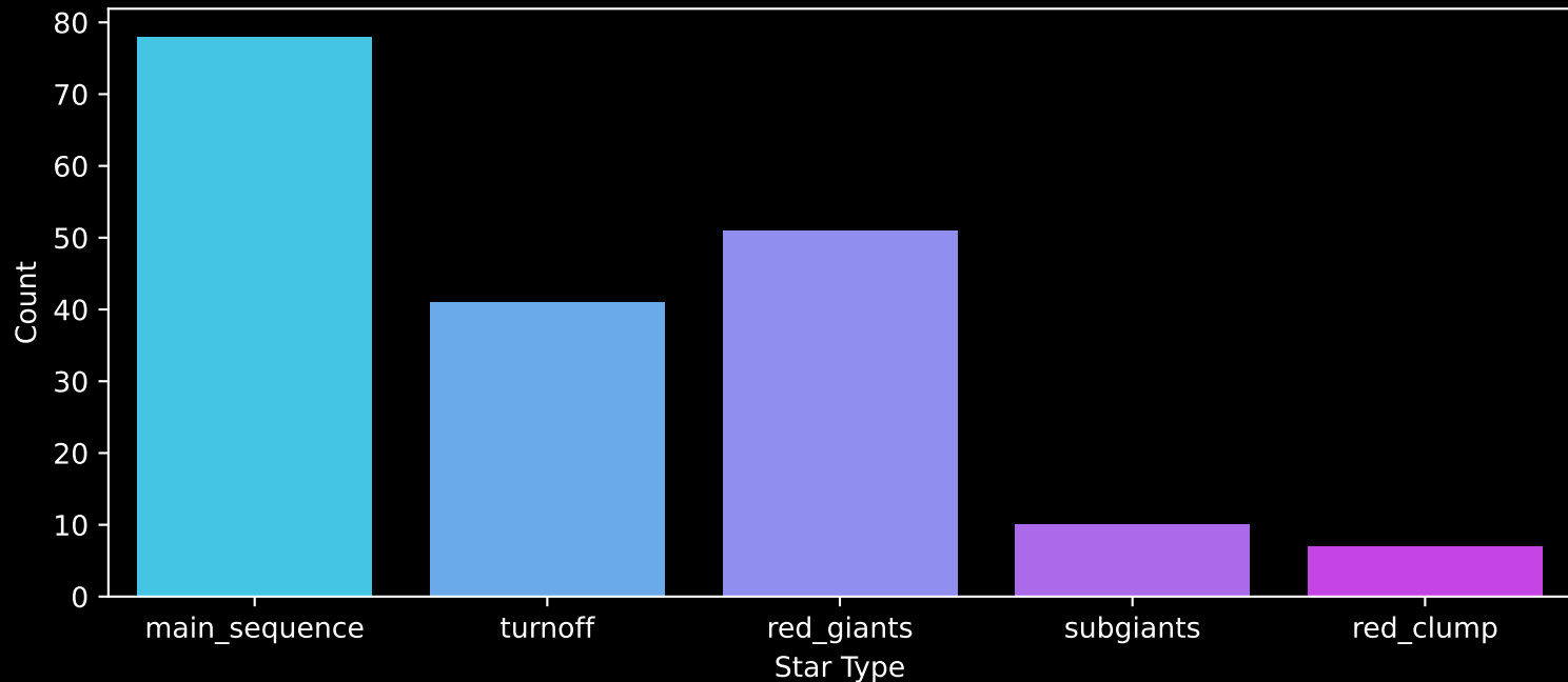
APOGEE DR17 Field: [175+31_MGA] Count plot of Star Type
