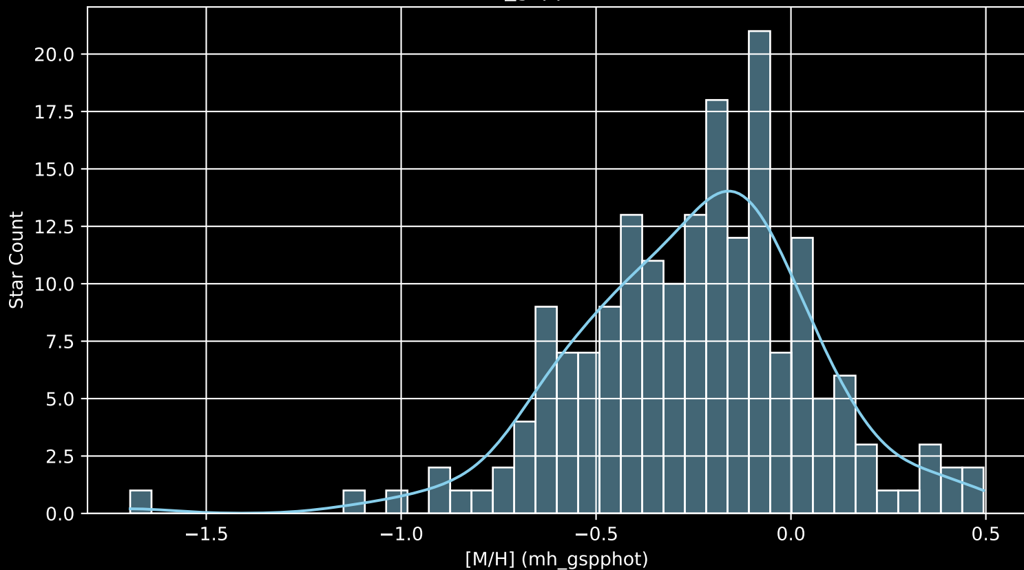
APOGEE DR17 Field: [175+31_MGA [M/H] (mh_gspphot) (n= 185)
