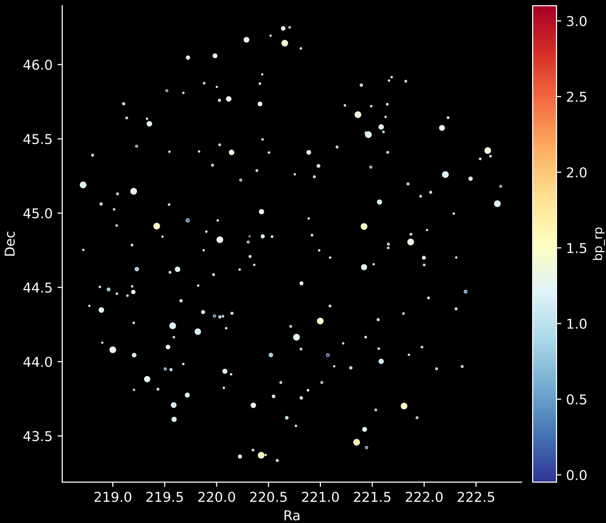
APOGEE DR17 Field: [175+31_MGA] Stars: 187
